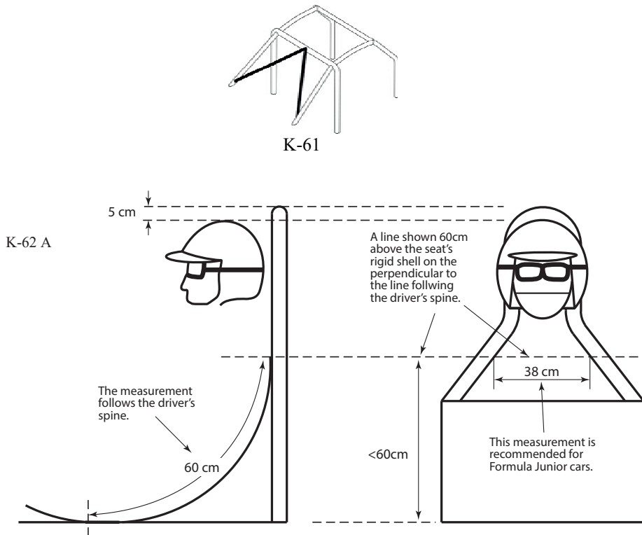
Fig 1. Roll over hoop dimensions
